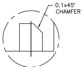
DETAIL A PIN 1 LEAD SCALE 50:1
