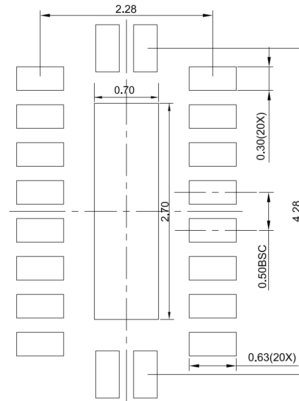
RECOMMENDED LAND PATTERN(unit:mm)
