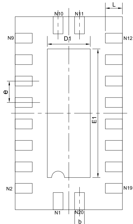
BOTTOM VIEW
