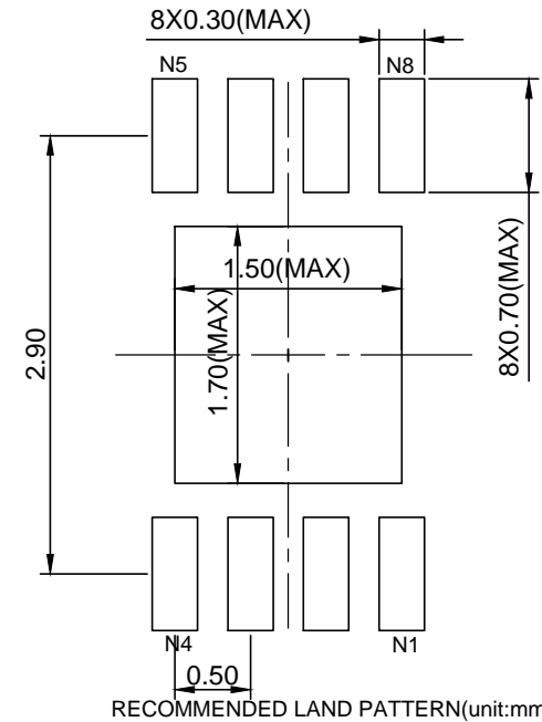
RECOMMENDED LAND PATTERN(unit:mm)
