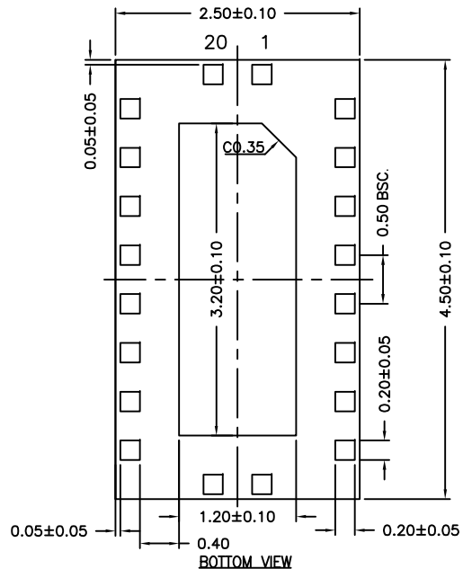
BOTTOM VIEW
