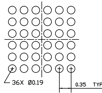
BOTTOMRECOMMEND LAND PATTERN VIEW
