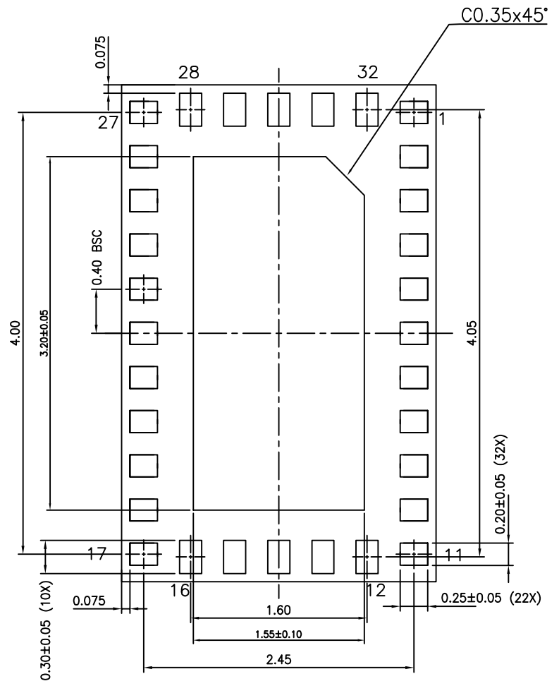
BOTTOM VIEW
