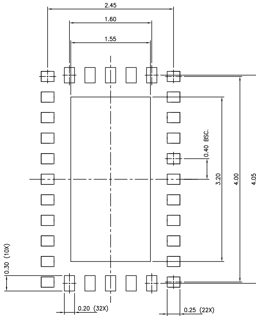
RECOMMENDED LAND PATTERN
