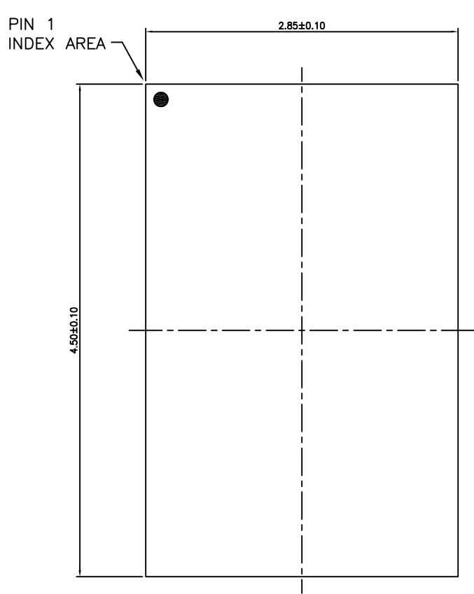
TOP VIEW
