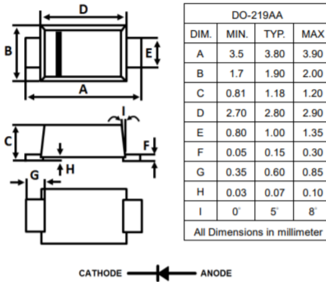
DO-219AA
