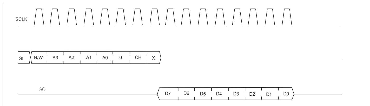
Figure 14. SPI Read
