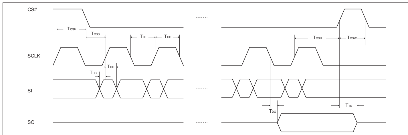
Figure 26. SPI-Bus Timing
