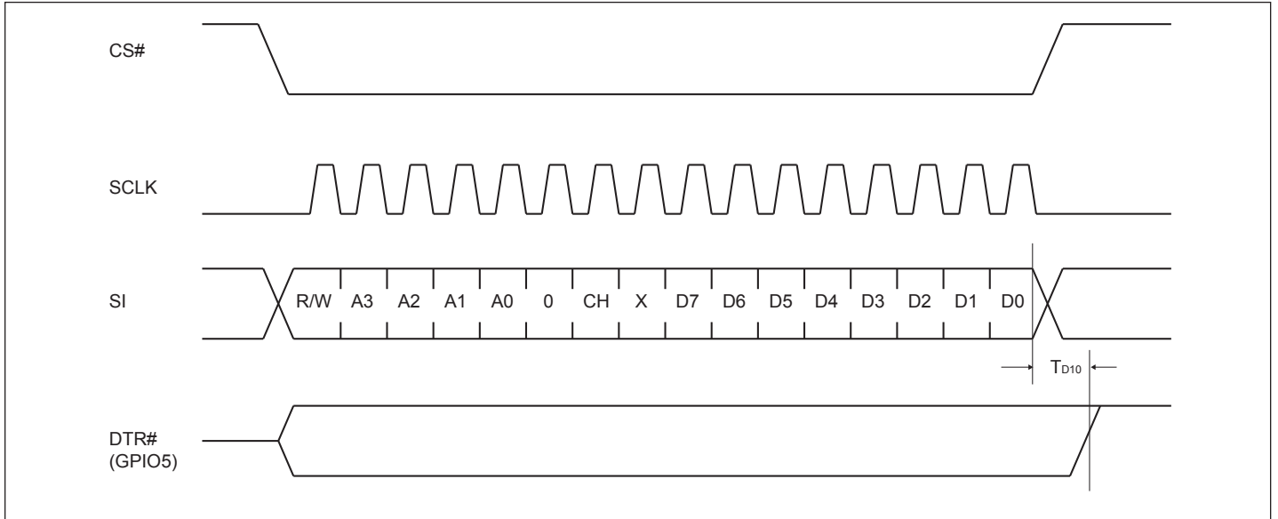
Figure 28. SPI Write MCR to DTR Output Switch
