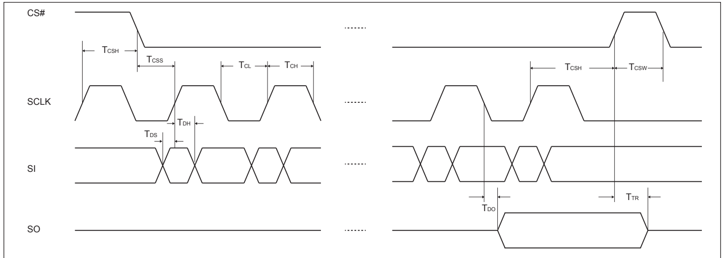
Figure 26. SPI-Bus Timing
