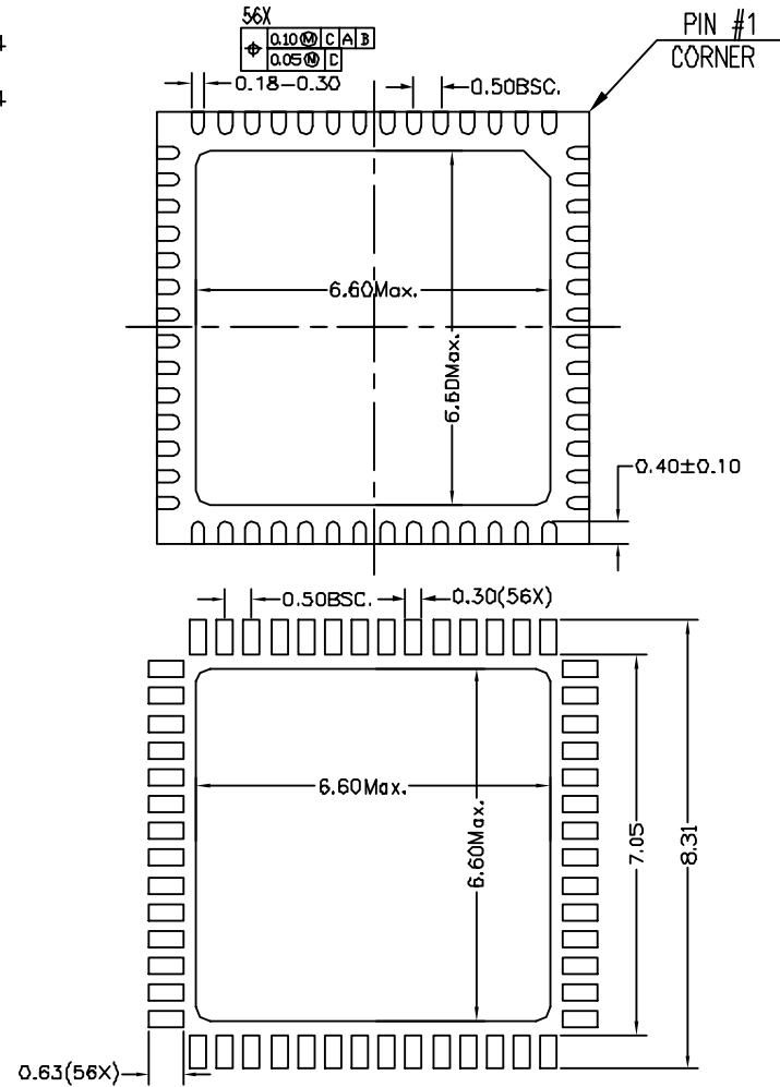
Recommended Land Pattern
