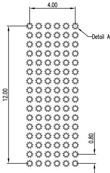
Recommended Land Pattern
