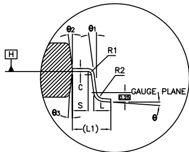
FIGURE 1 SECTION A-A
