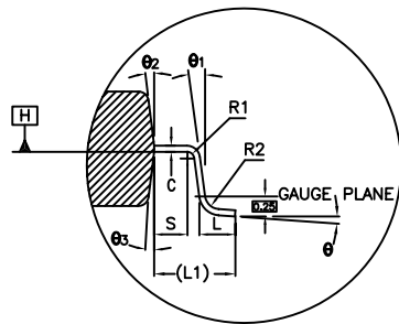
FIGURE 1 SECTION A-A
