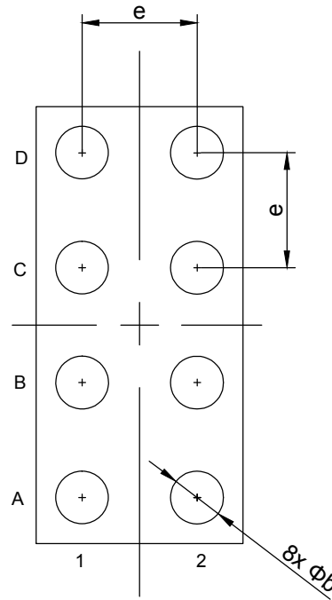
Bottom View
