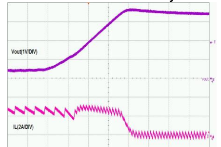
Time -20µs/div
