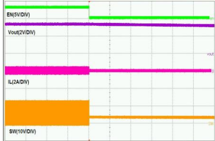
Time -10ms/div
